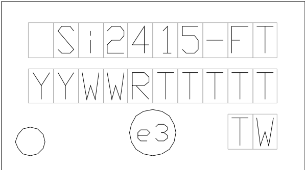
Figure 15. Si2415-D-FT Top Marking
